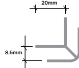
Type O external corner
