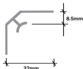
Type N internal corner
